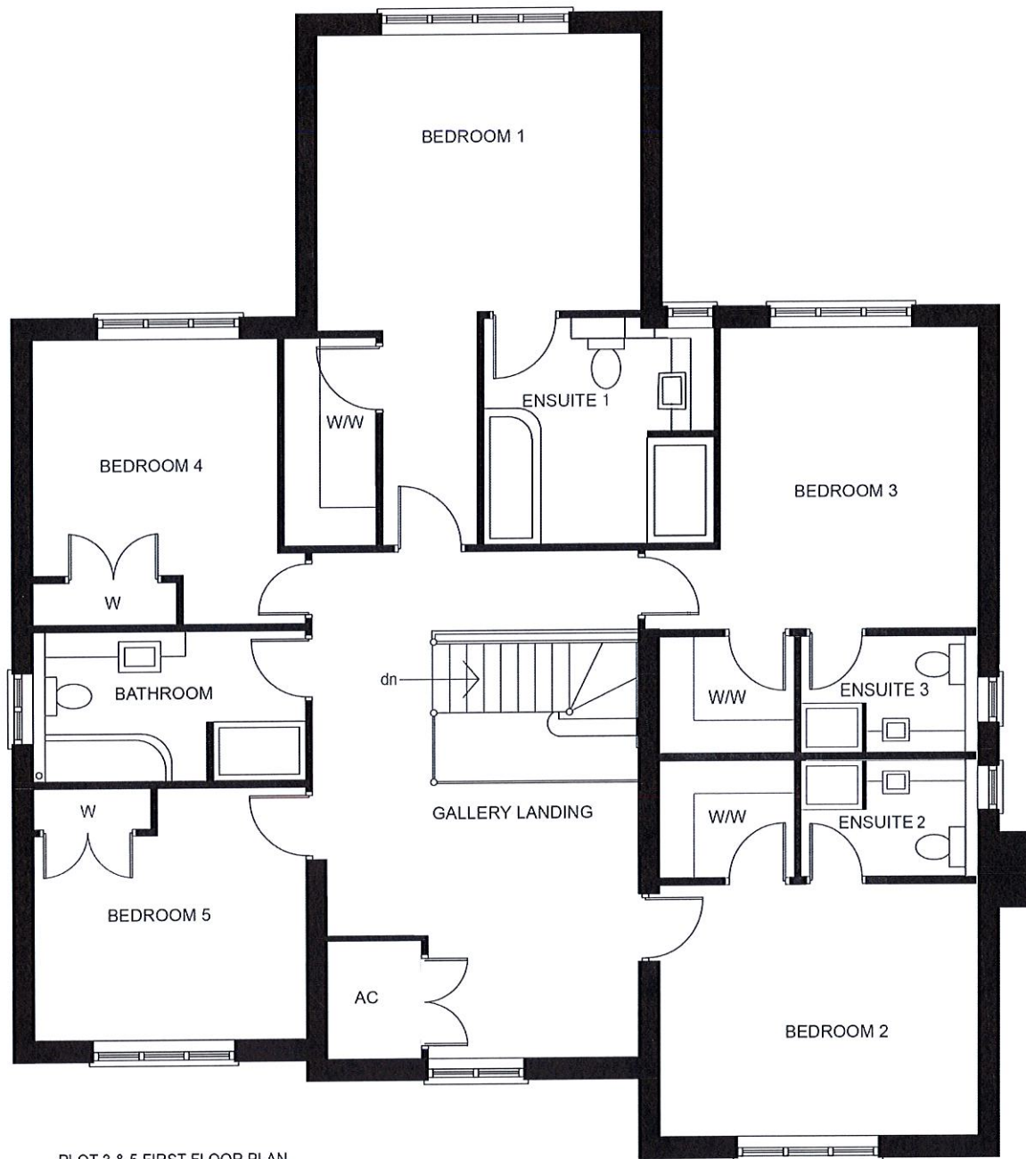
PLOT 3 & 5 FIRST FLOOR PLAN
