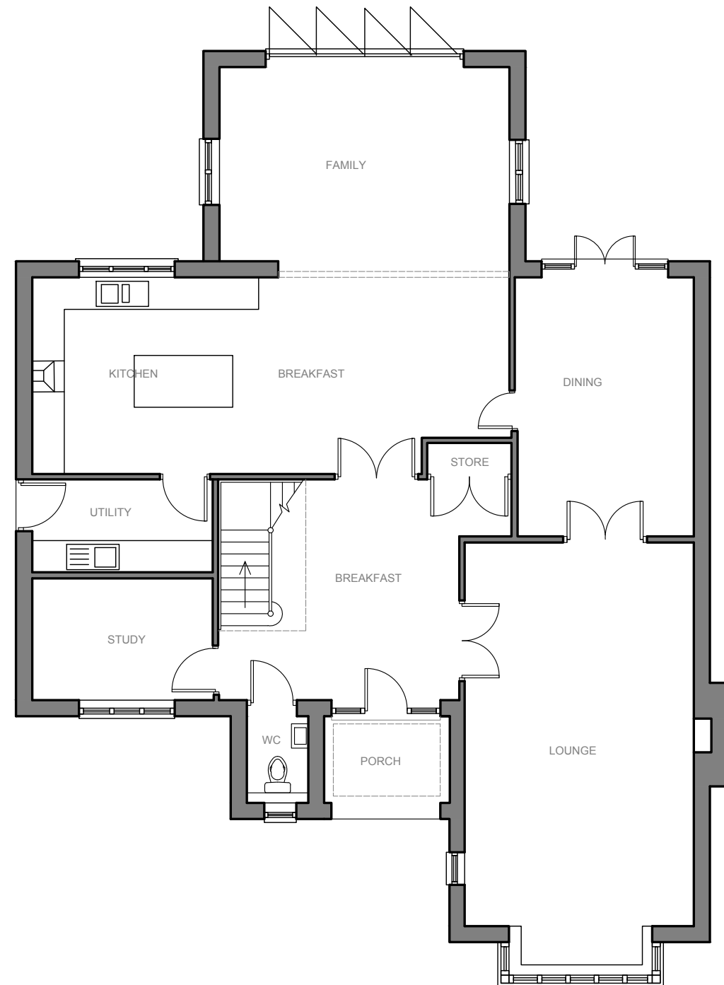
PLOT 1 GROUND FLOOR
