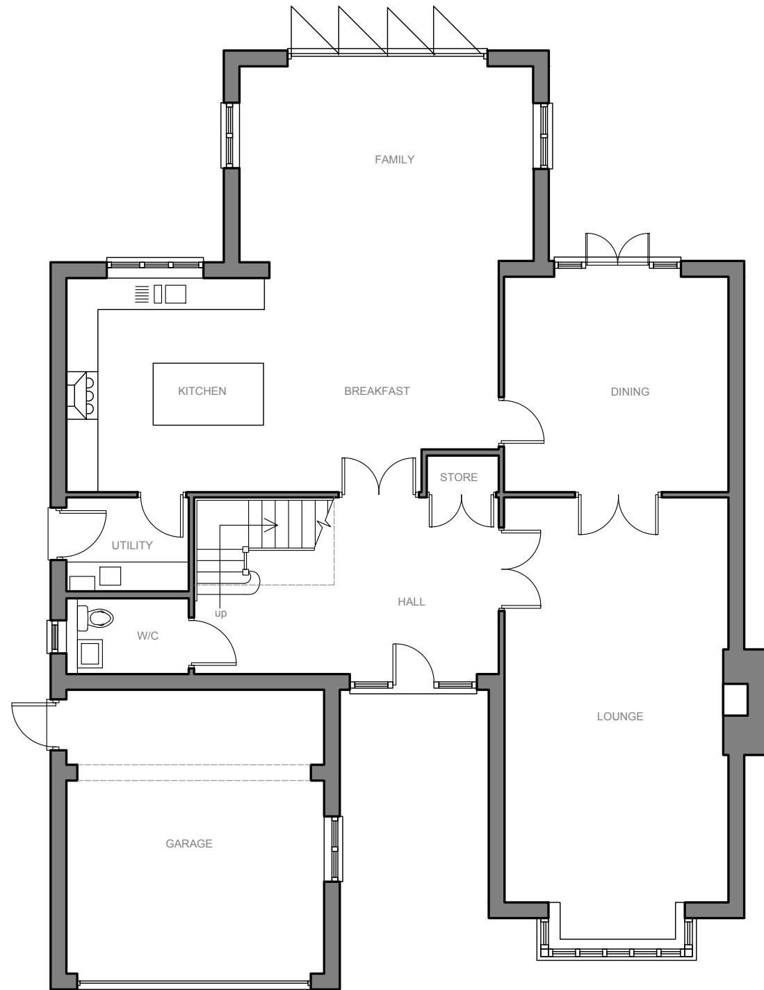
BURLINGTON HOUSE (PLOT 2) GROUND FLOOR
