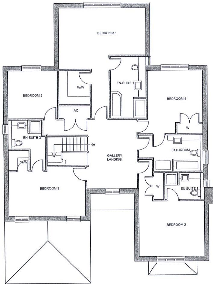
FIRST FLOOR PLAN PLOT 1: FAIRFIELD HOUSE 1B ST JOHNS DRIVE
