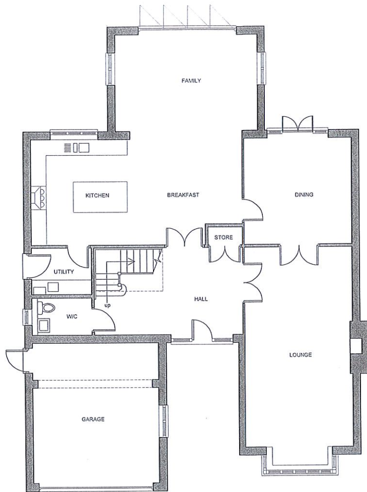
GROUND FLOOR PLAN PLOT 1: FAIRFIELD HOUSE 1B ST JOHNS DRIVE
