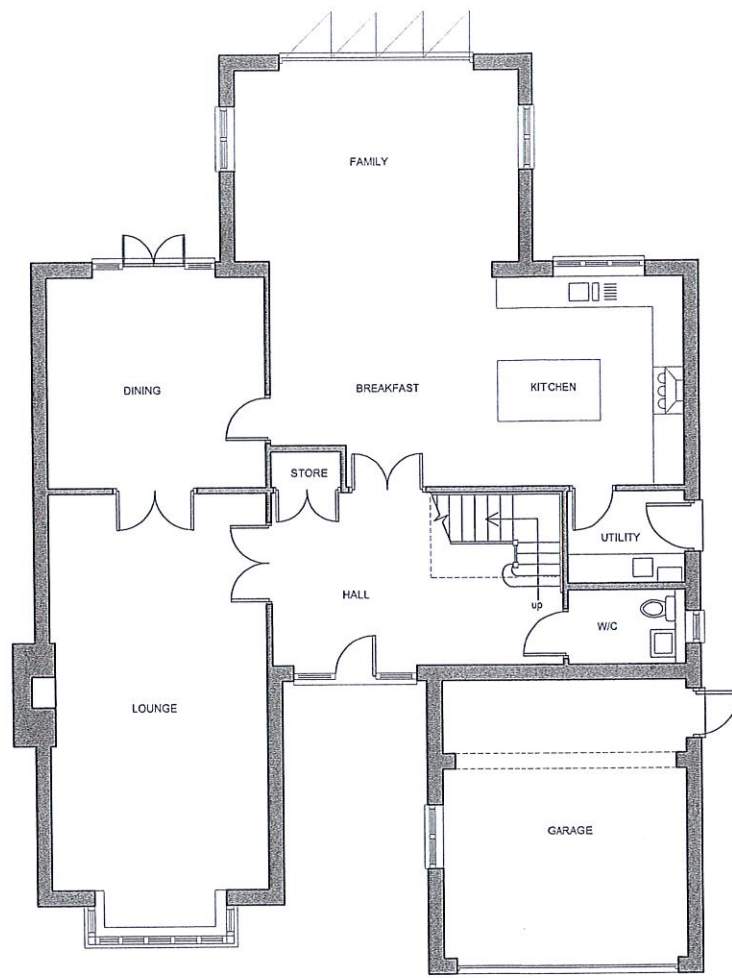
GROUND FLOOR PLAN PLOT 1: BURLINGTON HOUSE 48 ST JOHNS HILL
