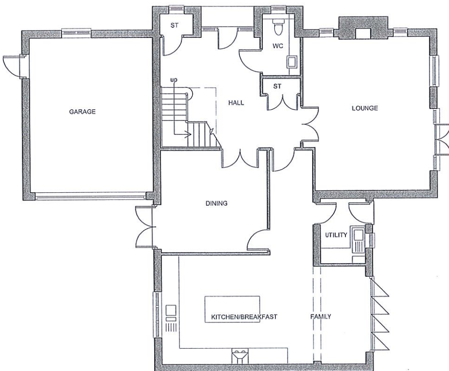
GROUND FLOOR PLAN PLOT 2: THORNFIELD HOUSE 48A ST JOHNS HILL
