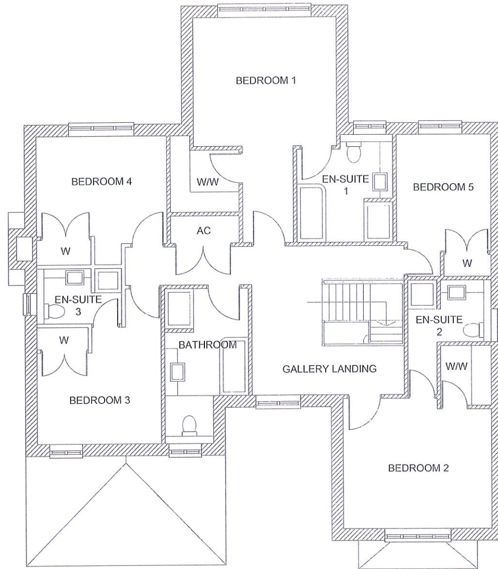
NO.3 FIRST FLOOR
