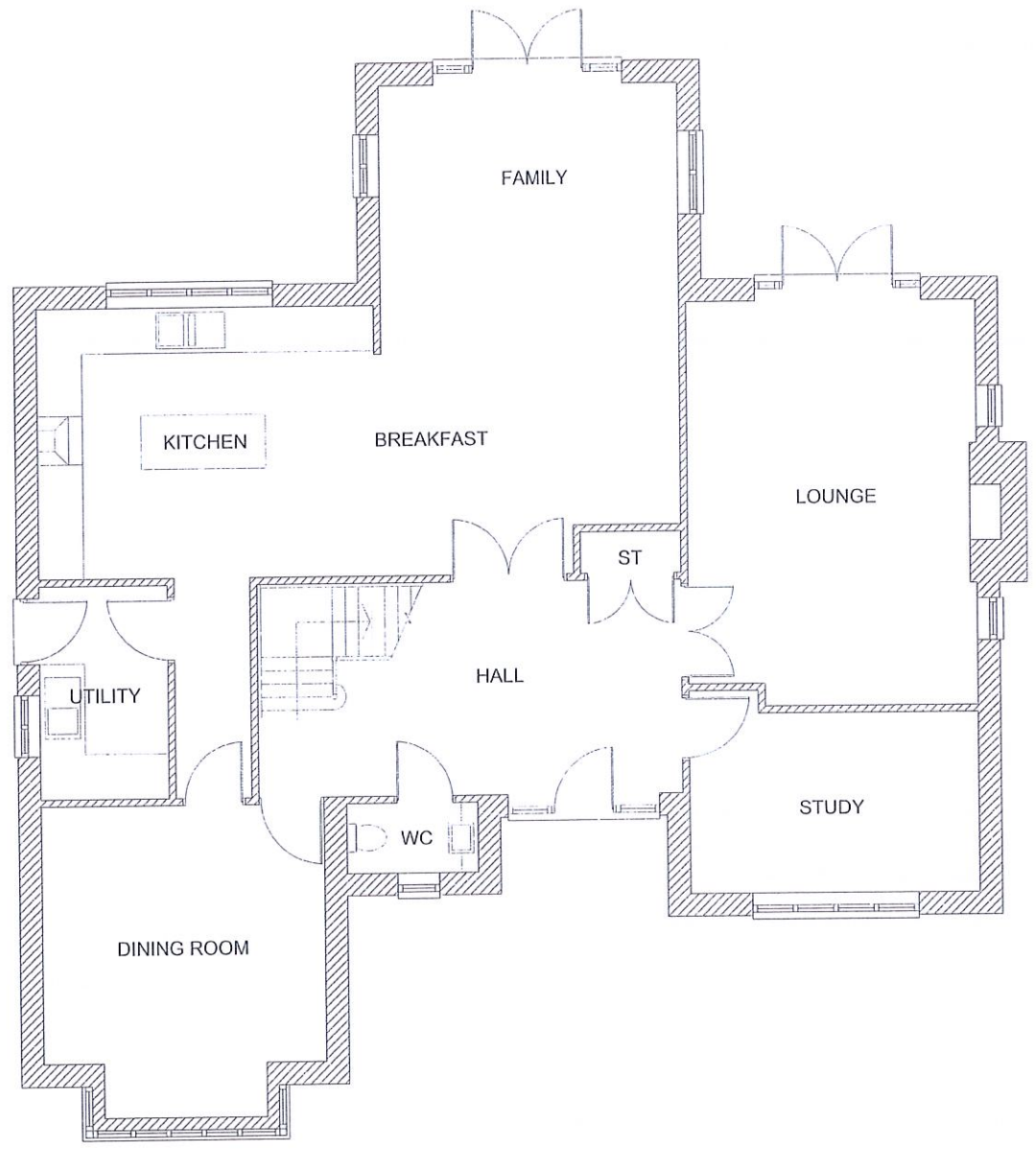
NO.7 GROUND FLOOR
